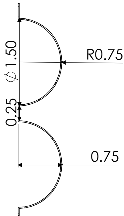
DETAIL C
