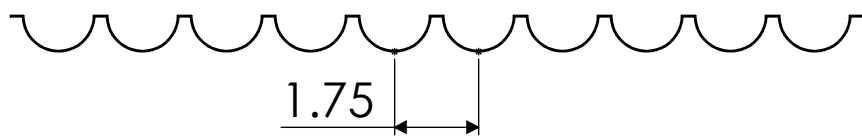
SECTION B
